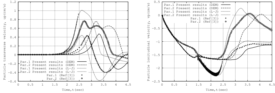
Figure 4.11: (a) Transverse velocity components of the two particles; (b) Longitudinal velocity components of the two particles.
