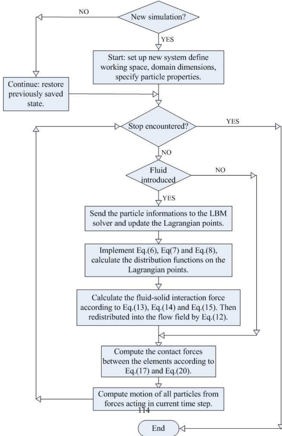
Figure 4.2: Flow chart for the computational sequence.
