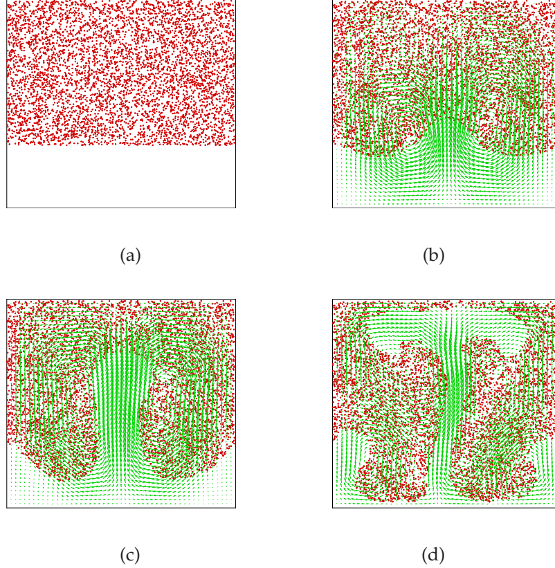
Figure 5.5: Instantaneous particle distribution with the fluid velocities at time (a) t = 0.0s , (b) t = 2.5s , (c) t = 5.0s , (d) t = 10.0s .
