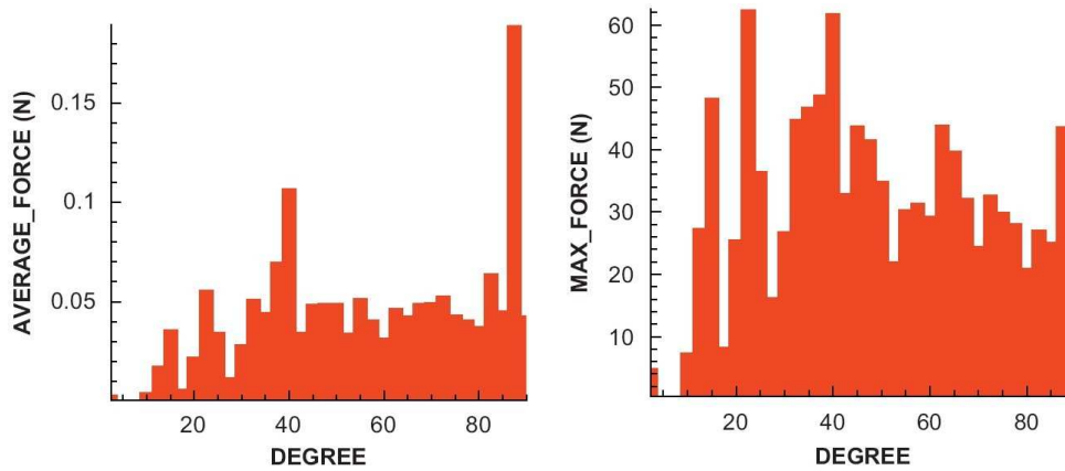
Figure 6.12: (a) average impact intensity distribution and (b) the max impact force distribution of the elbow from the bottom view.
