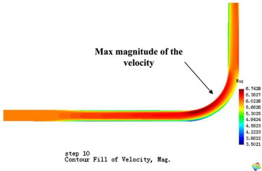
Figure 6.6: Velocity magnitude distribution profile of the particle-free slurry.
