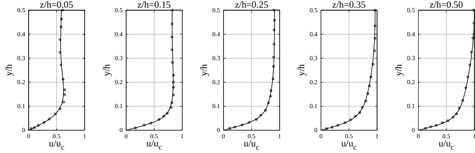
Figure 3.4: Quadrant-averaged profiles at five locations in the duct for the mean streamwise velocity. (—) Present DNS, (o) Gavrilakis [11].
