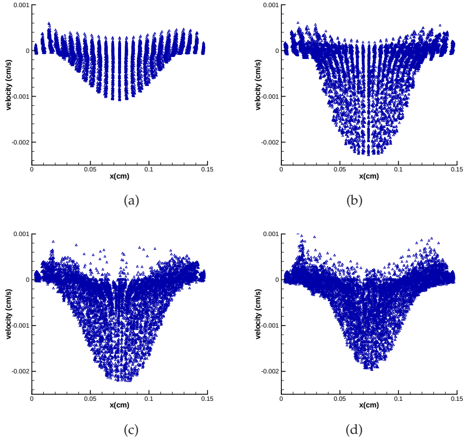
Figure 5.9: Particle deposition velocity along the x -direction at time (a) t = 2.5\text{s} , (b) t = 5.0\text{s} , (c) t = 7.5\text{s} , (d) t = 10.0\text{s} .
