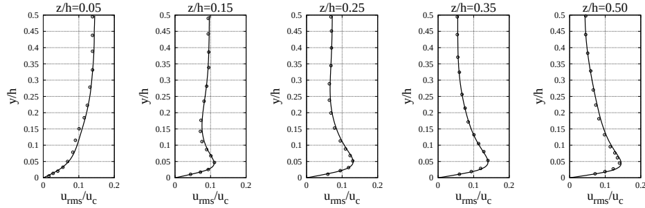
Figure 3.5: Quadrant-averaged profiles at five locations in the duct for rms fluctuations in streamwise velocity. (—) Present DNS, (o) Gavrilakis [11].
