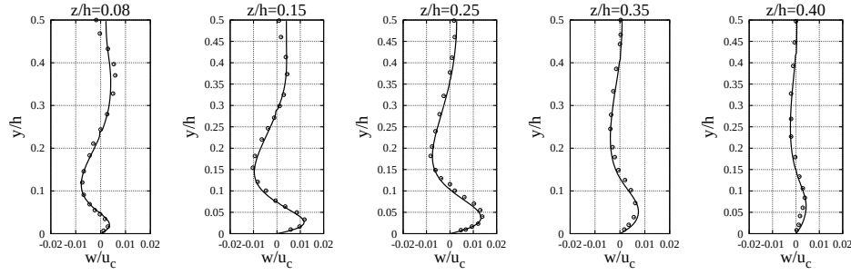
Figure 3.6: Quadrant-averaged profiles at five locations in the duct for the mean lateral velocity. (—) Present DNS, (o) Gavrilakis [11].
