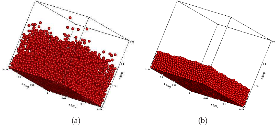
Figure 5.12: (a) Positions of the 8125 particles at time t = 50.0s and (b) the final distribution.
