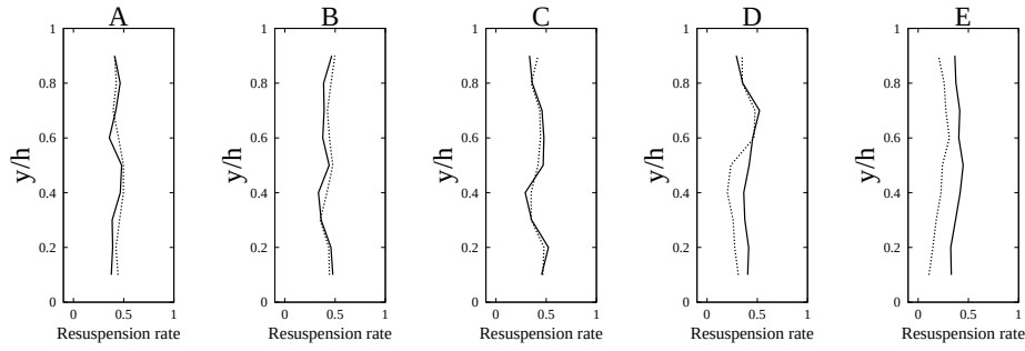
Figure 3.20: Particle resuspension rate in the z -direction for 50 \mu m particles. Solid line: with collisions. Dashed line: without collisions.
