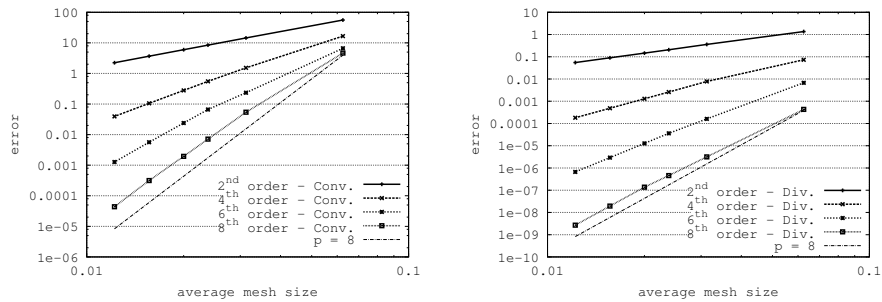
Figure 3.1: Numerical errors versus mesh size for convective (left) and divergence (right) operators for second-, fourth-, sixth- and eighth-order discretizations.
