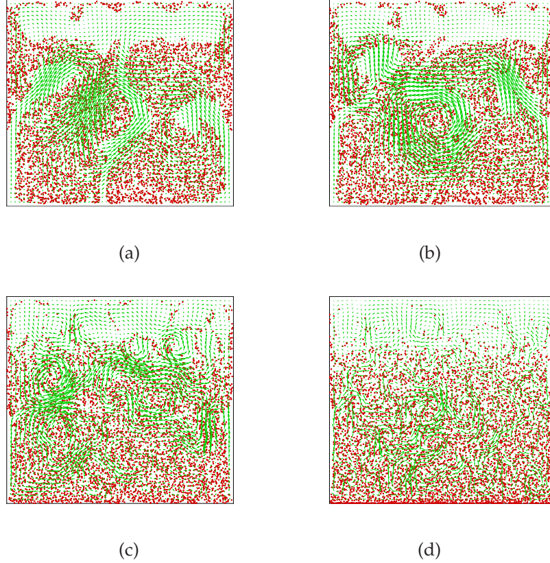
Figure 5.6: Instantaneous particle distribution with the fluid velocities at time (a) t = 20.0s , (b) t = 25.0s , (c) t = 50.0s , (d) t = 100.0s .
