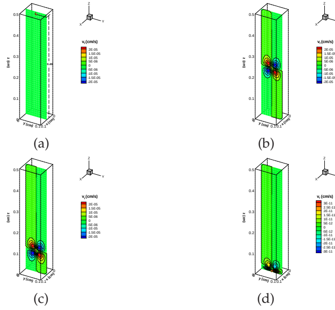
Figure 5.4: Instantaneous height of the 100\mu m particle with contour plots for v_f at time (a) t = 0.0s , (b) t = 45.0s , (c) t = 67.5s , (d) t = 90.0s .
